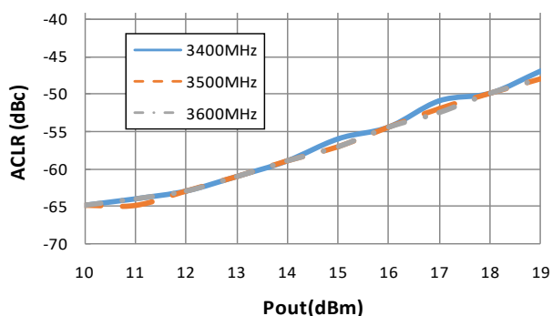
LTE BAND42 ACLR vs. Pout
