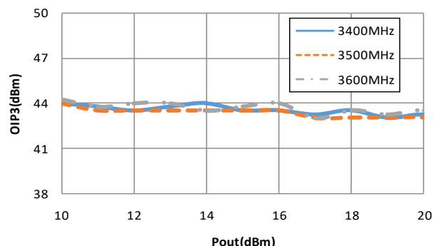
LTE BAND42 OIP3 vs. Pout
