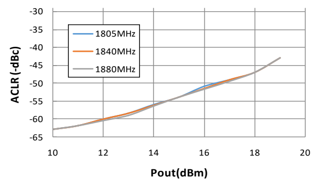
LTE BAND3 ACLR vs. Pout
