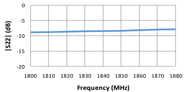
Output Return Loss vs. Frequency
