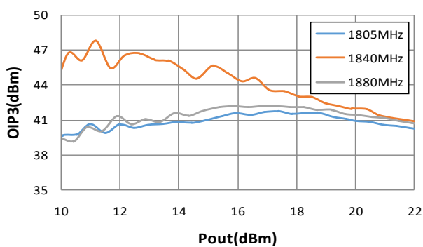
LTE BAND3 OIP3 vs. Pout
