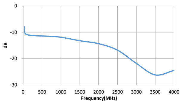
S11
