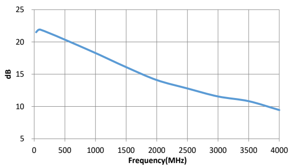
Gain
