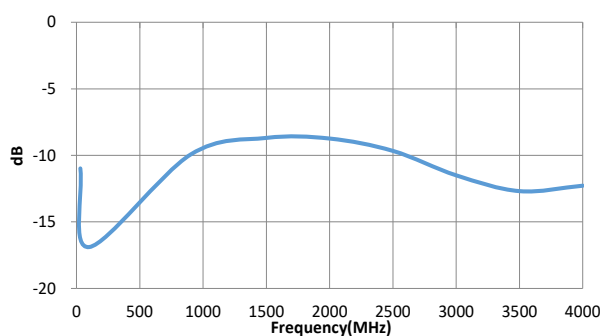
S22
