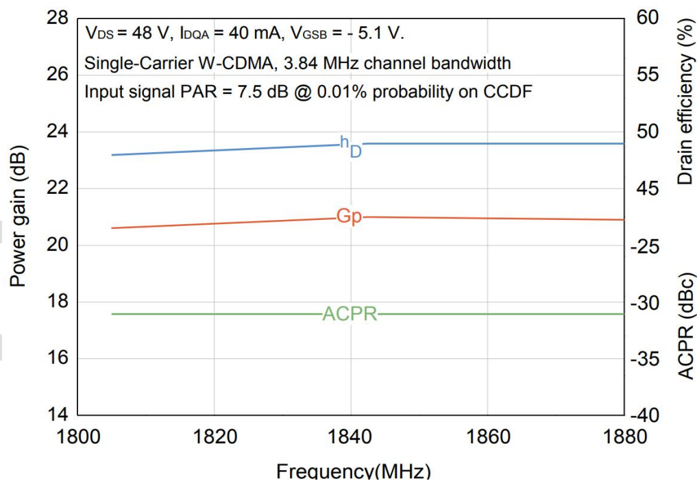
Power gain, Drain efficiency, ACPR vs. Frequency Single-Carrier W-CDMA @ Pout = 7.1 Watts Avg.
